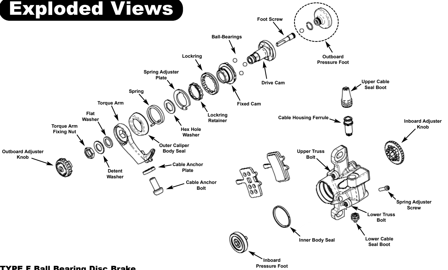
TYPE F Ball Bearing Disc Brake
